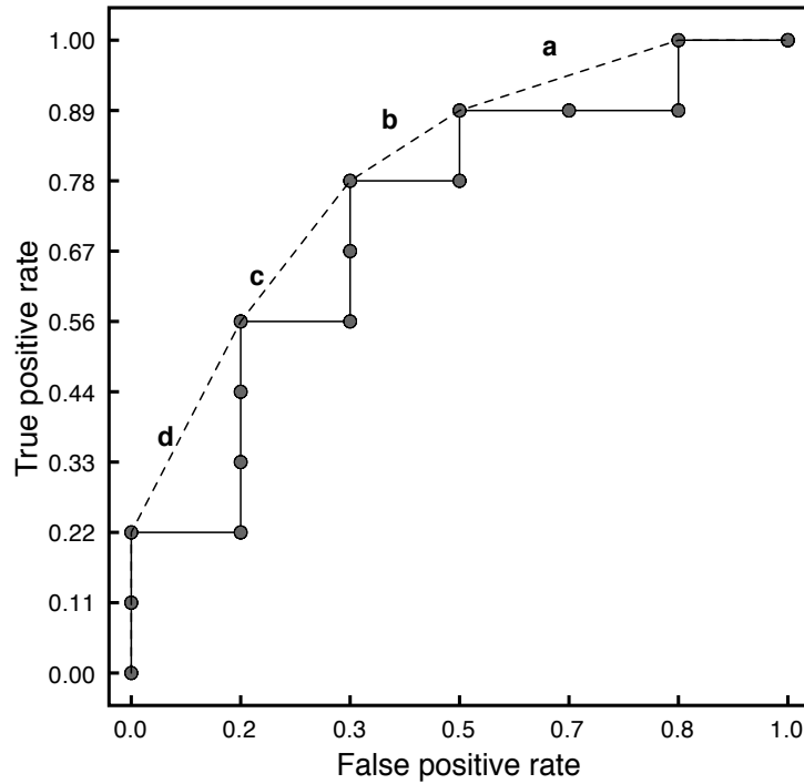
Figure 2. The instances of table I in ROC space
