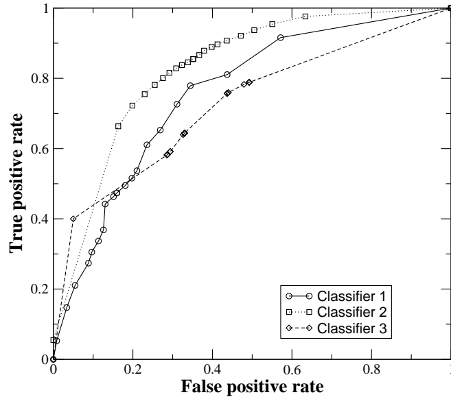
Figure 1. An ROC graph of three scoring classifiers
